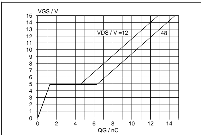
Fig. 13. Typical turn-on gate-charge characteristics. V_{GS} = f(Q_G) ; conditions: I_D = 2.7 A; parameter V_{DS}
