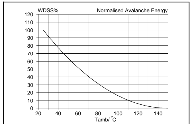
Fig. 15. Normalised avalanche energy rating. W_{DSS}\% = f(T_{amb}) ; conditions: I_D = 2.7 A
