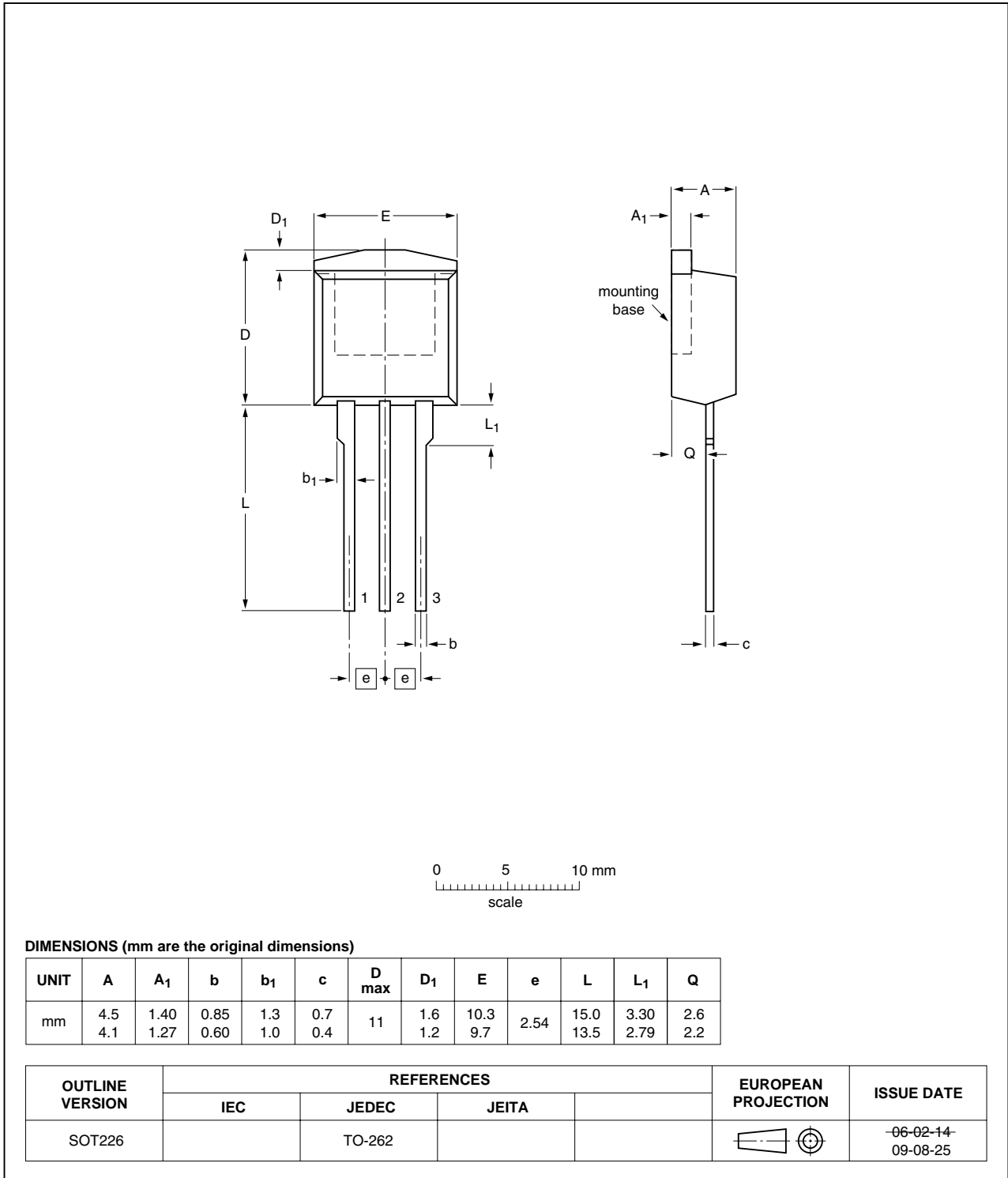
Fig 6. Package outline SOT226 (I2PAK)
