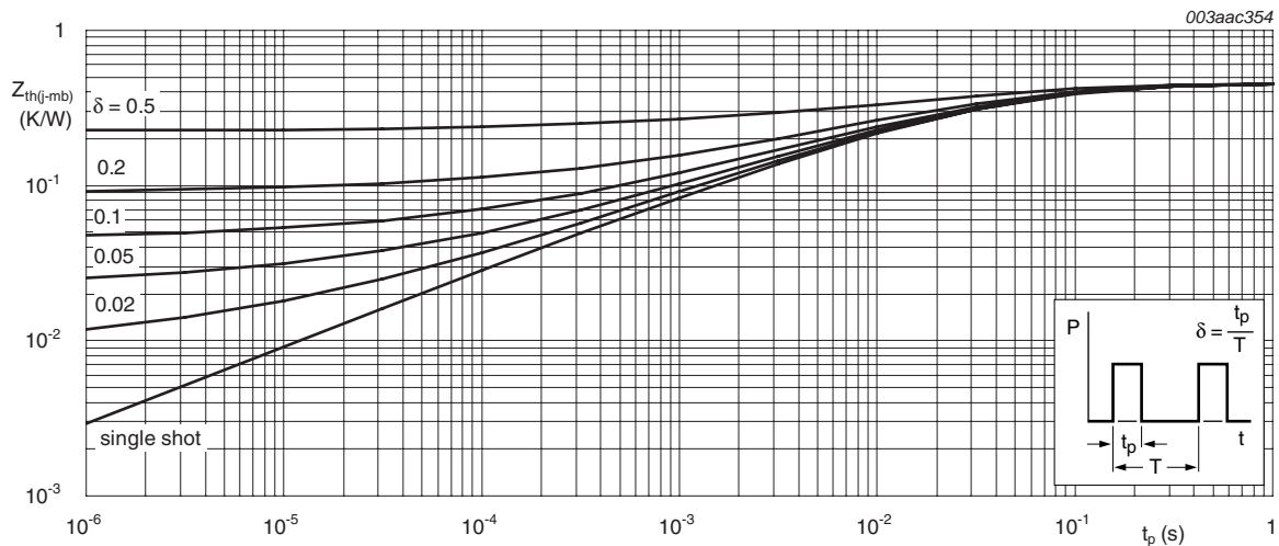
Fig 3. Transient thermal impedance from junction to mounting base as a function of pulse duration
