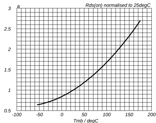
Fig.10. Normalised drain-source on-state resistance. R_{DS(ON)}/R_{DS(ON)25\text{ }^{\circ}\text{C}} = f(T_j)
