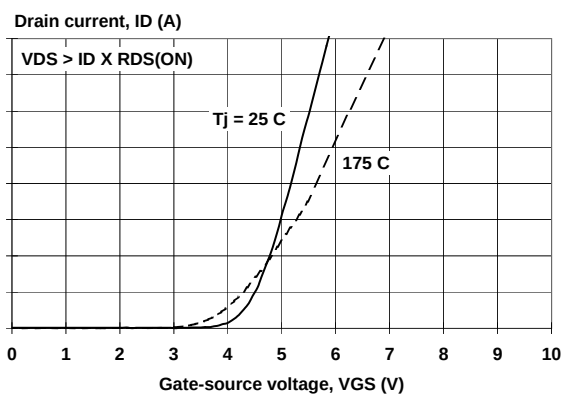
Fig.8. Typical transfer characteristics. I_D = f(V_{GS})
