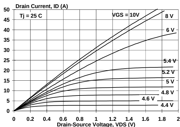
Fig.5. Typical output characteristics, T_j = 25\text{ }^{\circ}\text{C} . I_D = f(V_{DS})
