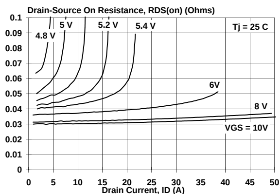
Fig.6. Typical on-state resistance, T_j = 25\text{ }^{\circ}\text{C} . R_{DS(ON)} = f(I_D)
