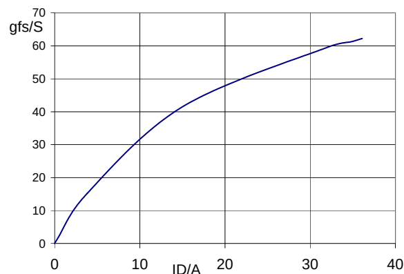
Fig.9. Typical transconductance, T_j = 25\text{ }^{\circ}\text{C} . g_{fs} = f(I_D)
