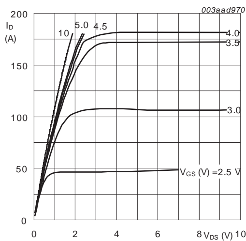
Fig 6. Output characterizations; drain current as a function of drain-source voltage; typical values.
