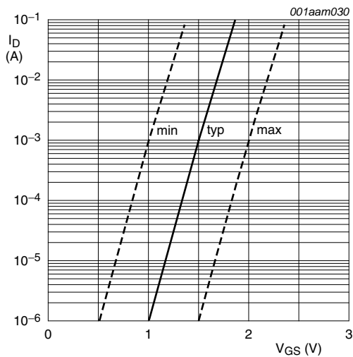
Fig 12. Transfer characteristics; drain current as a function of gate-source voltage; typical values, FET1 and FET2
