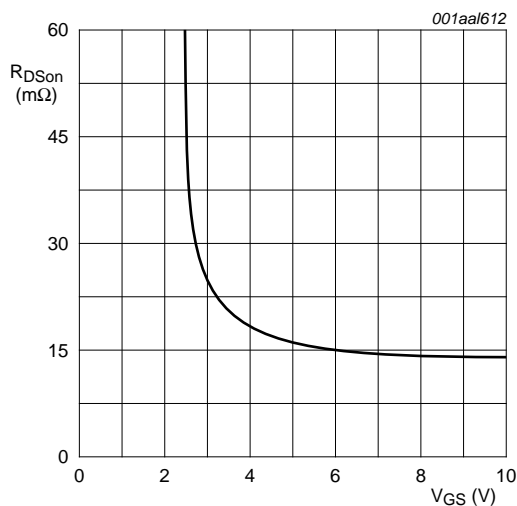
Fig 9. Drain-source on-state resistance as a function of gate-source voltage; typical values, FET1 and FET2
