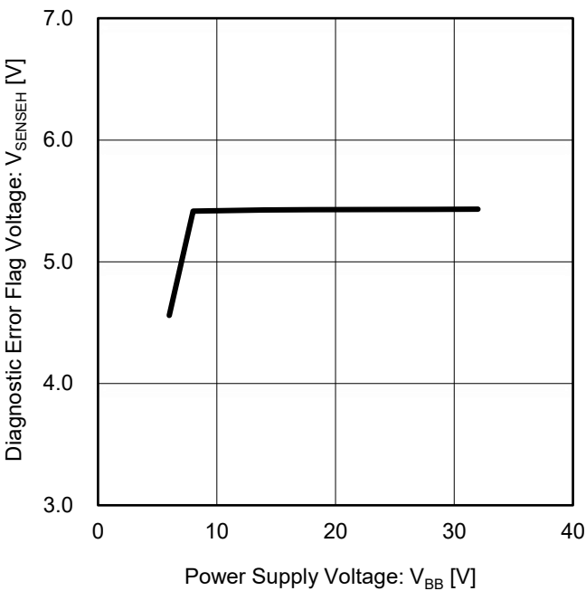
Figure 35. Diagnostic Error Flag Voltage vs Power Supply Voltage
