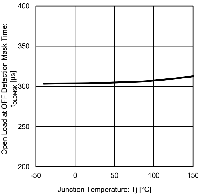
Figure 43. Open Load at OFF Detection Mask Time vs Junction Temperature
