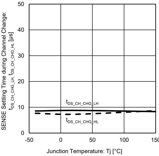
Figure 41. SENSE Settling Time during Channel Change vs Junction Temperature
