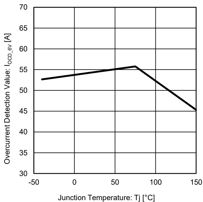
Figure 31. Overcurrent Detection Value vs Junction Temperature
