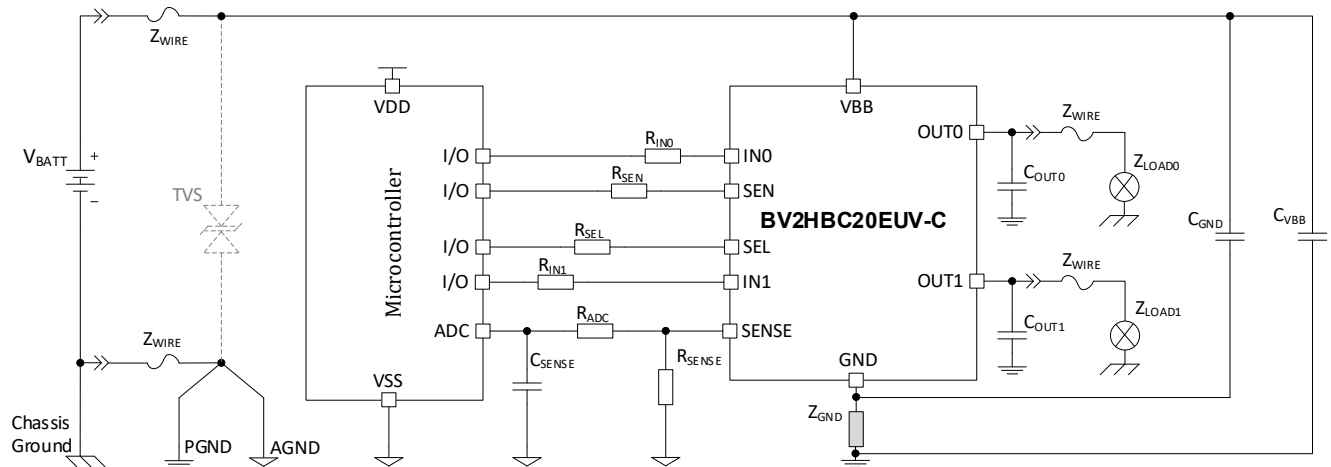
Figure 74. Application Schematic
