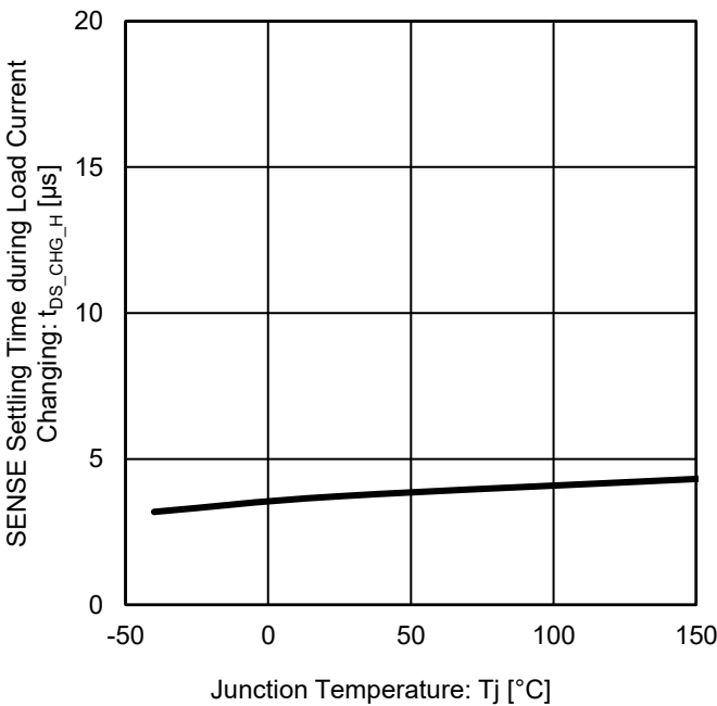
Figure 39. SENSE Settling Time during Load Current Changing vs Junction Temperature
