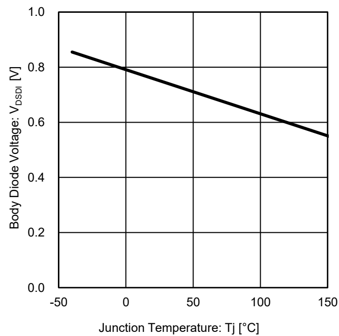
Figure 29. Body Diode Voltage vs Junction Temperature
