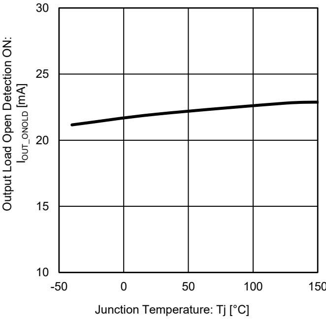
Figure 45. Output Load Open Detection ON vs Junction Temperature
