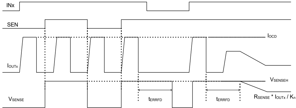
Figure 68. Overcurrent Protection
