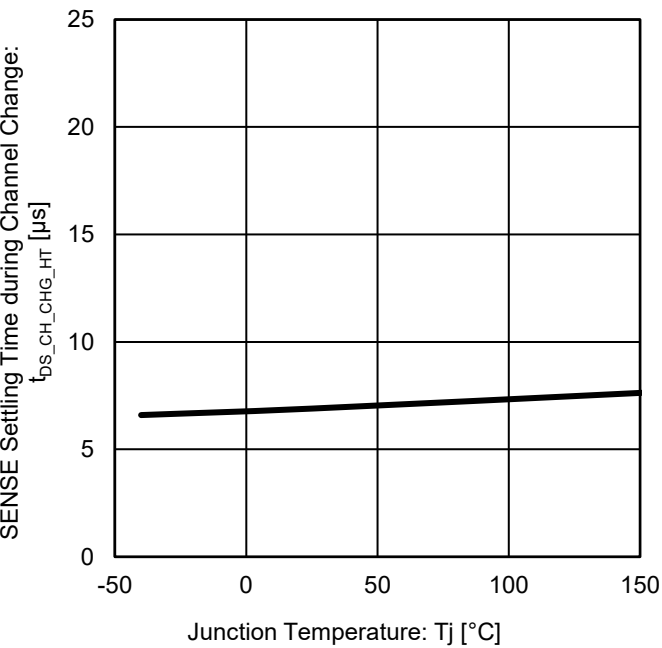
Figure 42. SENSE Settling Time during Channel Change vs Junction Temperature
