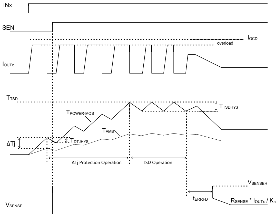
Figure 67. Overtemperature Protection
