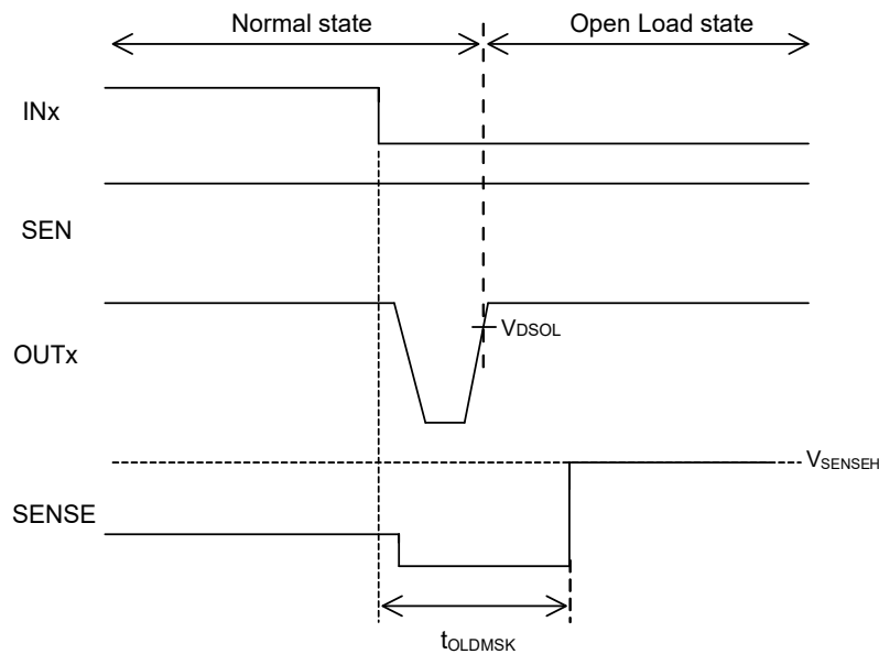
Figure 72. Open Load Mask Timing Chart
