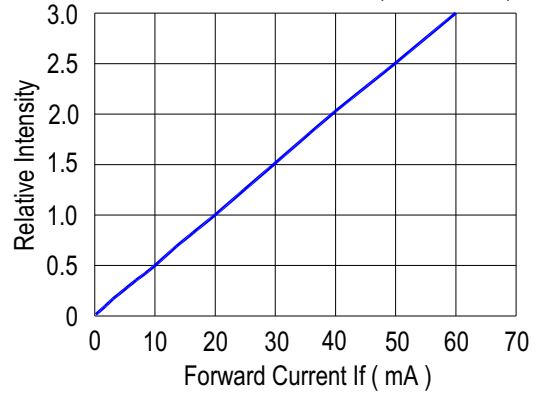
FIG. 2 Relative Intensity vs. Forward Current (Ta = 25 °C)
