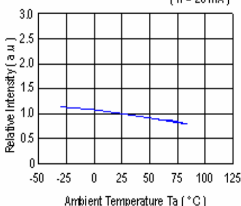
FIG. 4 Relative Intensity vs. Temperature ( I_f = 20\text{ mA} )
