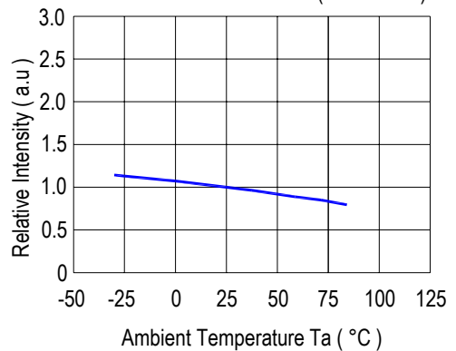
FIG. 4 Relative Intensity vs. Temperature ( I_f = 20\text{ mA} )
