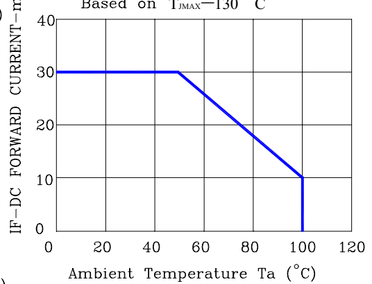
FIG. 6 Maximum Forward Current vs. Ambient Temperature. Derating Based on T_{JMAX}=130^{\circ}C
