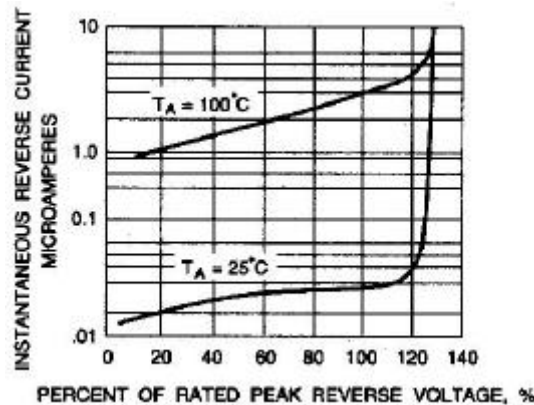
Fig. 5-TYPICAL REVERSE CHARACTERISTICS
