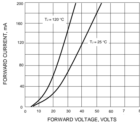
FIG.4 - MAXIMUM FORWARD CHARACTERISTICS
