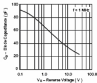
Diode Capacitance vs. Reverse Voltage
