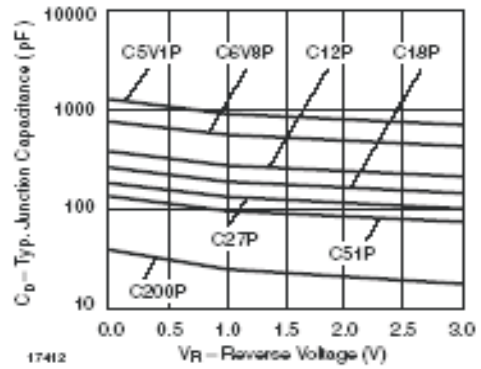
FIG.2- TYP. DIODE CAPACITANCE vs REVERSE VOLTAGE
