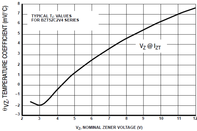
Figure 1. Temperature Coefficients (Temperature Range -55^{\circ}\text{C} to +150^{\circ}\text{C} )
