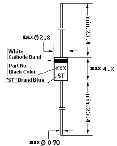
Glass Case JEDEC DO-41
