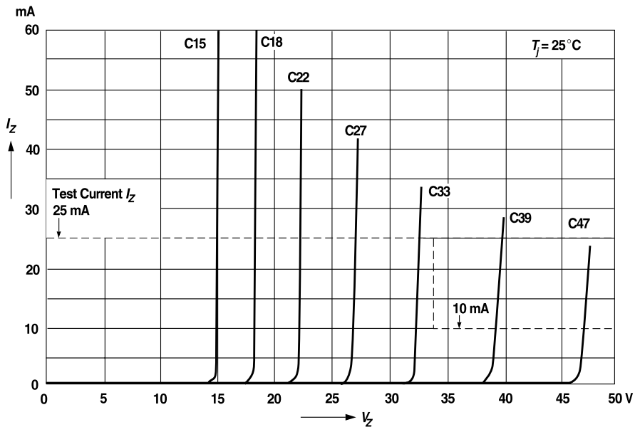
Figure 7. Breakdown Characteristics
