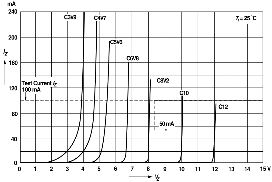
Figure 6. Breakdown Characteristics
