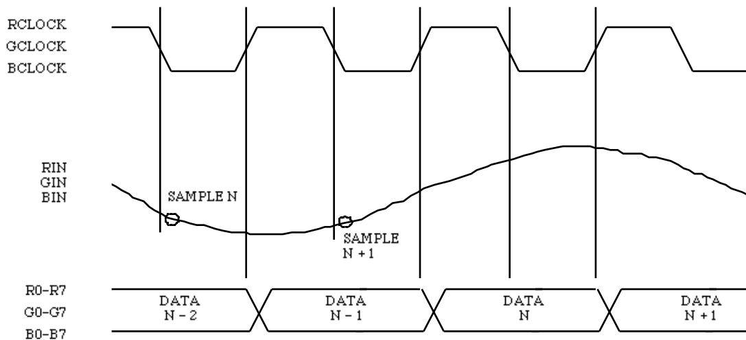
Figure 2. Input/Output Timing.
