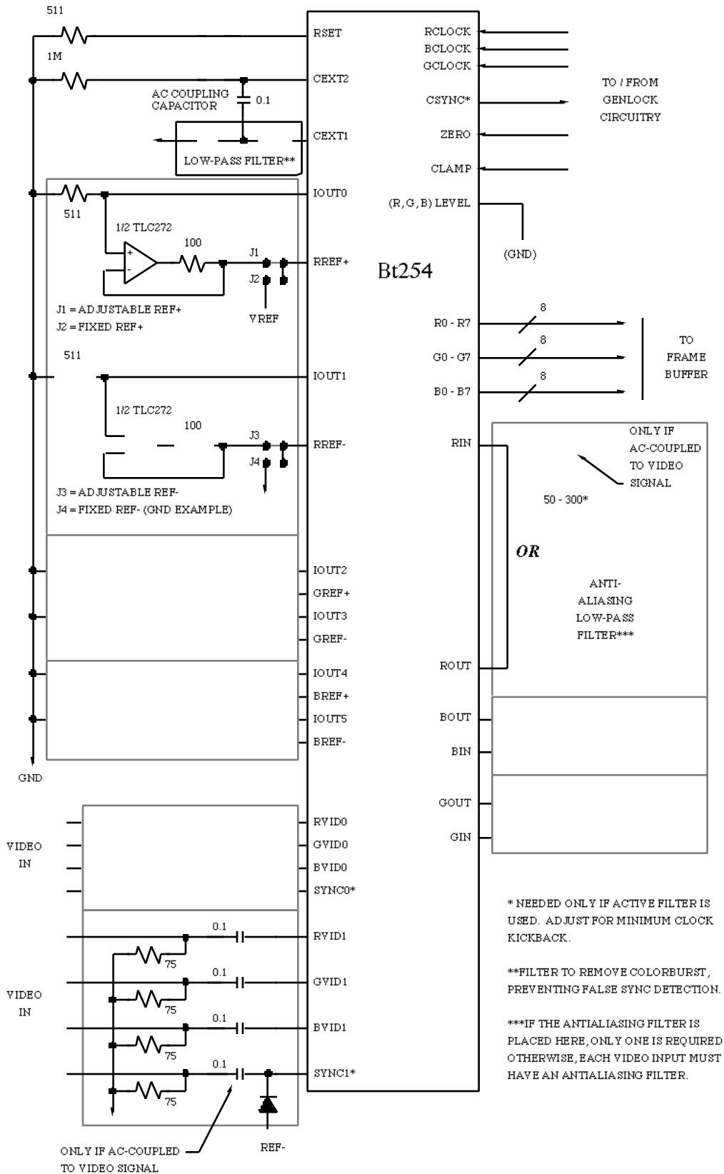
Figure 3. Typical Bt254 External Circuitry.
