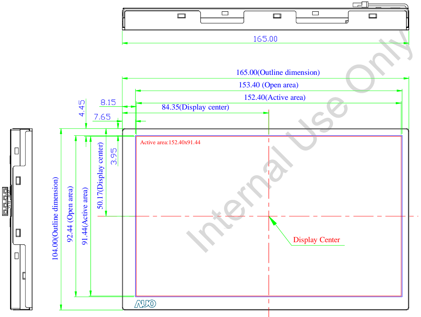
Figure 6. Front View
