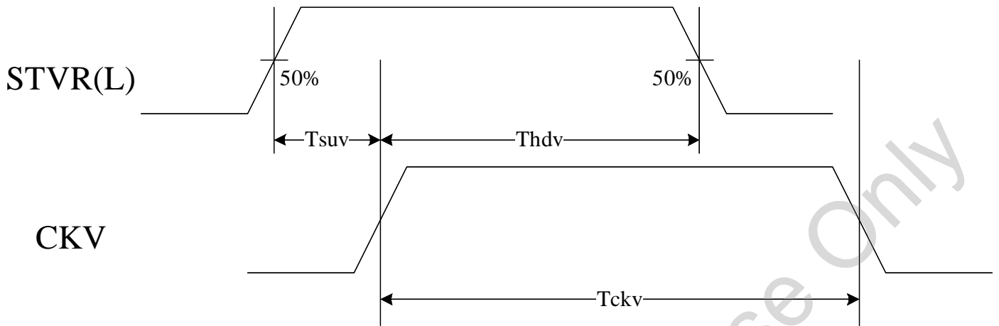
Figure 4. Vertical shift clock timing
