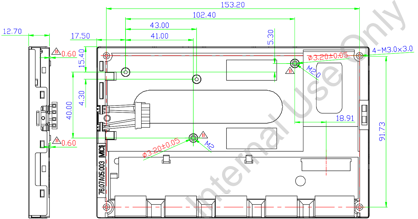
Figure 7. Back View
