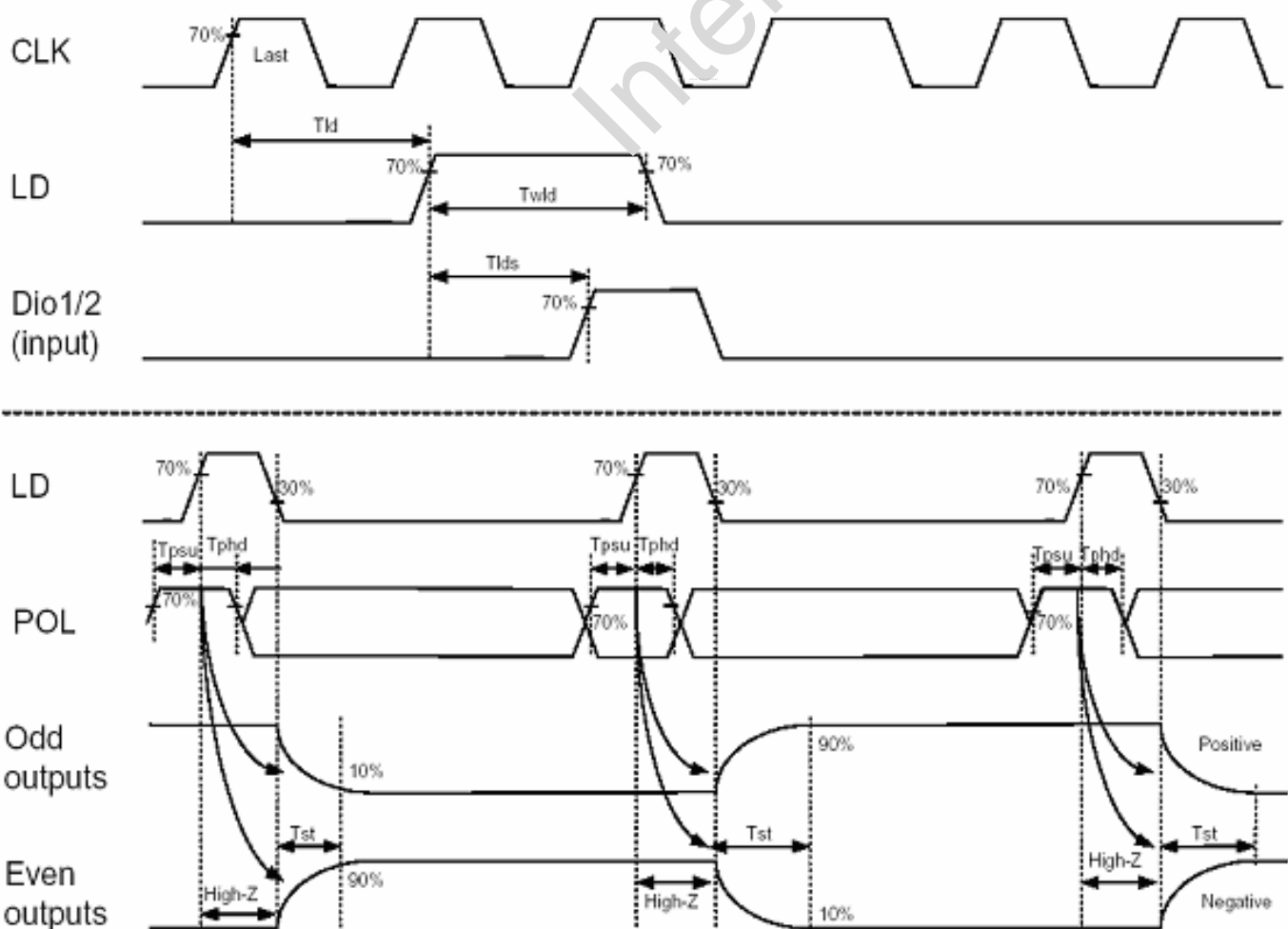
Figure 3. Horizontal Timing
