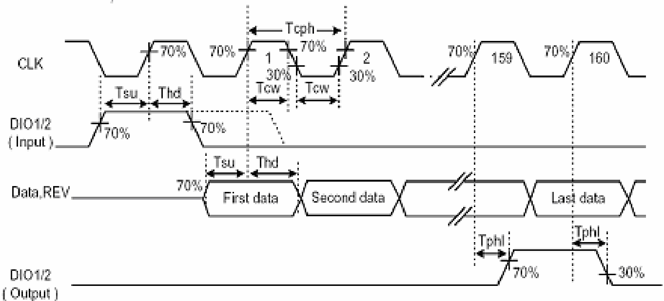
Figure 1. Operation Mode 1
