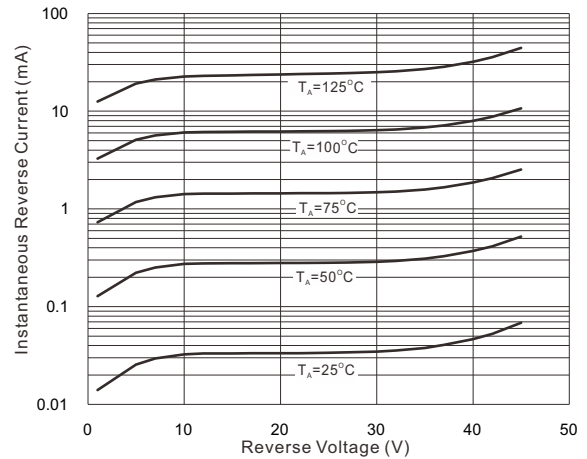
Fig. 2 - Reverse Characteristics
