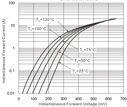
Fig. 1 - Instantaneous Forward Characteristics
