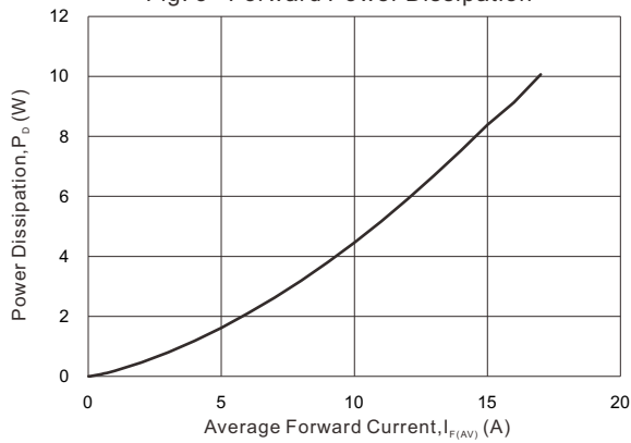
Fig. 3 - Forward Power Dissipation
