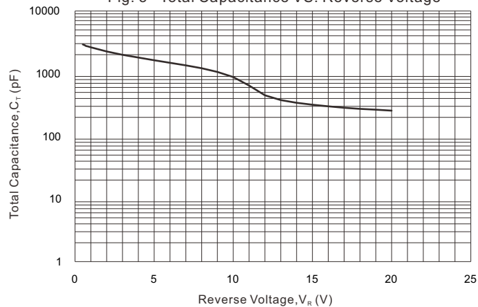
Fig. 5 - Total Capacitance VS. Reverse Voltage
