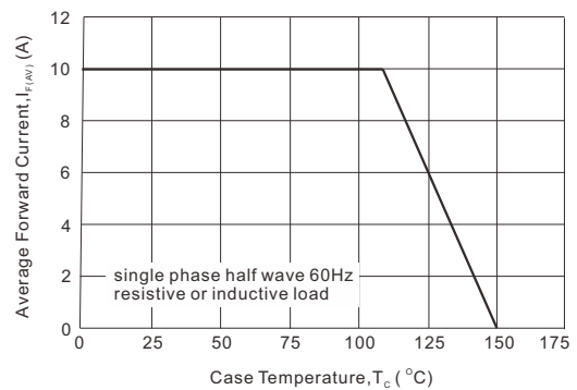
Fig. 4 - Forward Current Derating Curve
