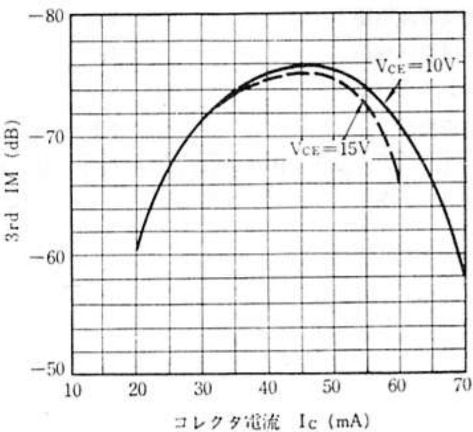
3rd ORDER IM DISTORTION vs. COLLECTOR CURRENT
