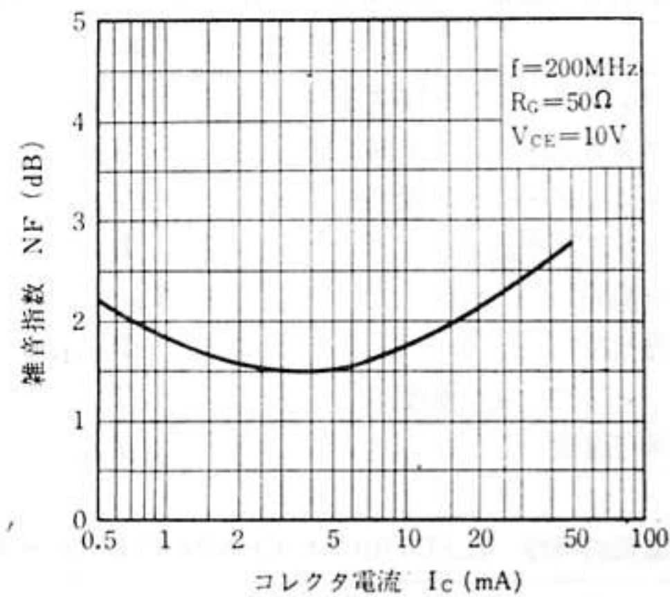
NOISE FIGURE vs. COLLECTOR CURRENT
