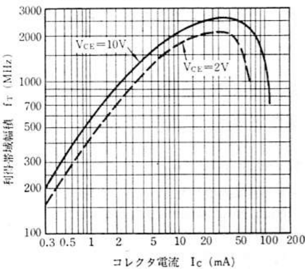
GAIN BANDWIDTH PRODUCT vs. COLLECTOR CURRENT
