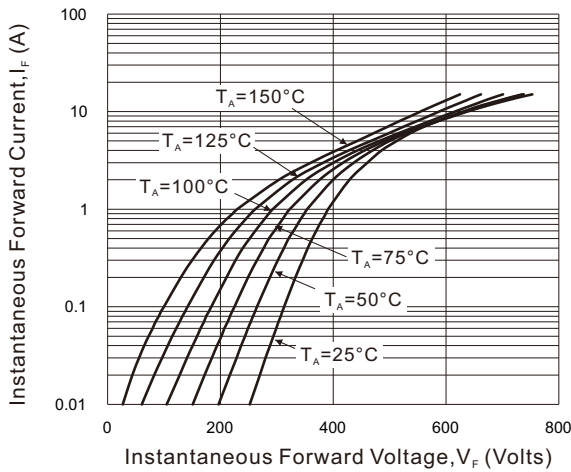
Fig. 1 - Instantaneous Forward Characteristics (per diode)
