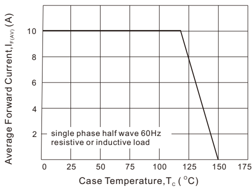
Fig. 3 - Forward Current Derating Curve (per diode)
