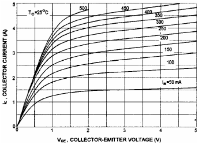
Fig.3 Static Characteristic
