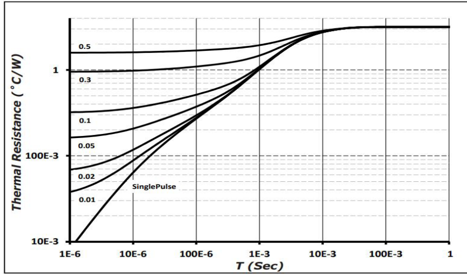
Figure 8 Transient Thermal Impedance
