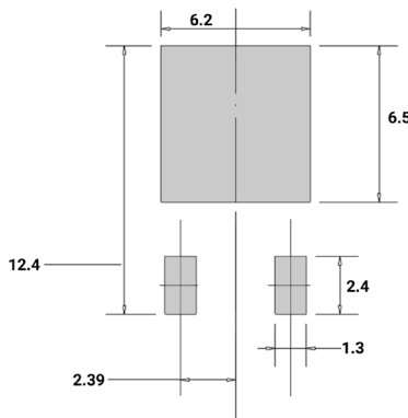
TO-252-2
