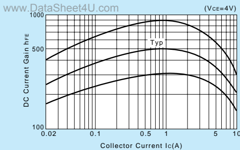
h_{FE}-I_C Characteristics (Typical)
