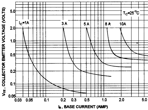
"ON" VOLTAGES
