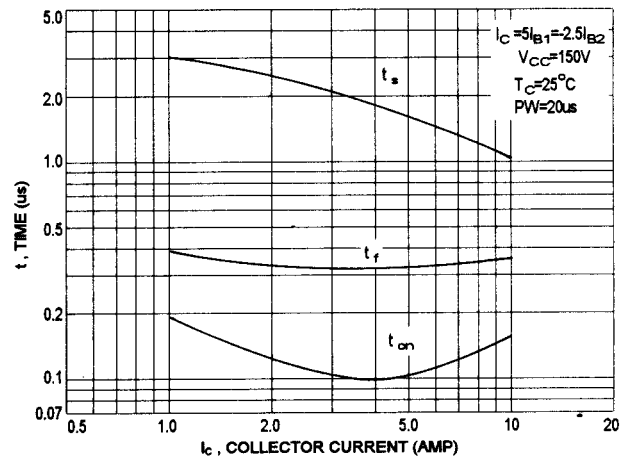
SWITCHING TIME
