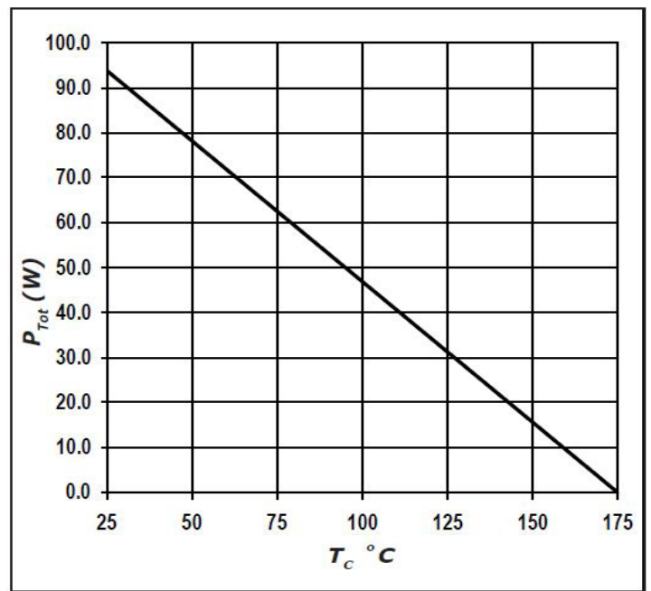
Figure 4 Power Derating
