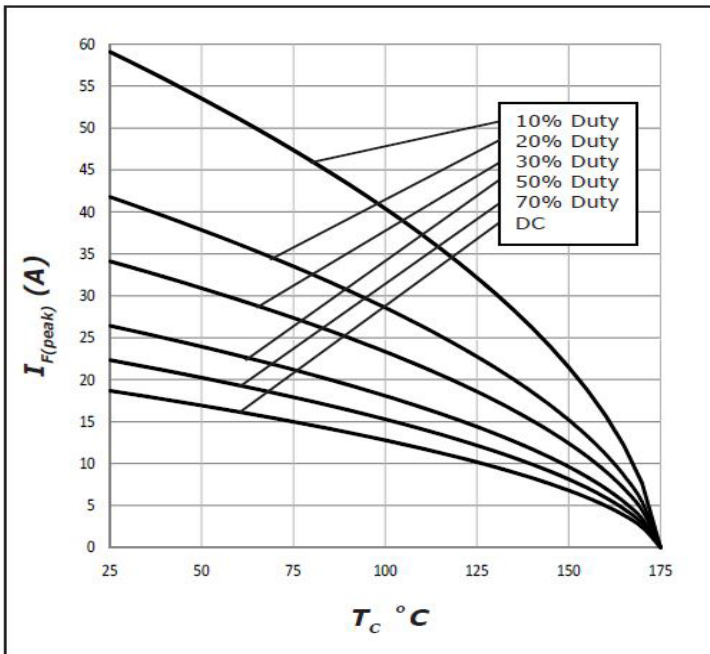
Figure 3 Current Derating
