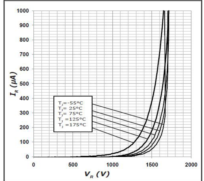
Figure 2 Reverse Characteristics
