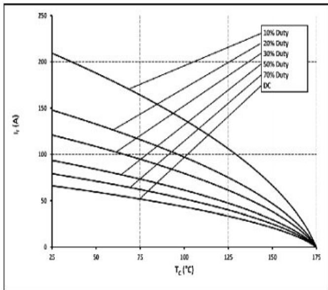
Figure 3 Current Derating
