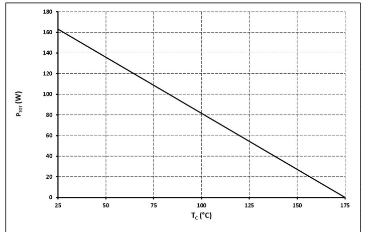
Figure 4 Power Derating
