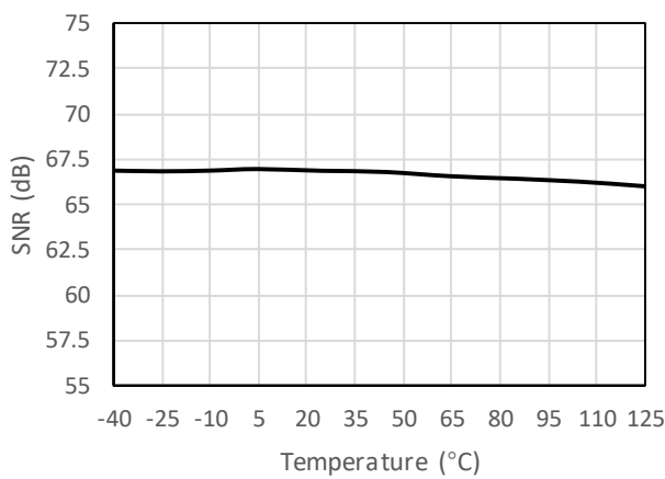
Figure 7-11 SNR vs Temperature @ f_{IN} = 10 \text{ kHz}
