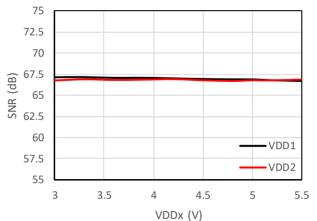
Figure 7-12 SNR vs Supply Voltage @ f_{IN} = 10 \text{ kHz}
