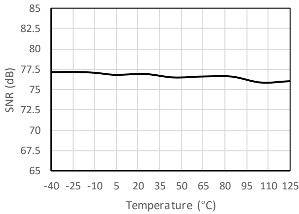
Figure 7-9 SNR vs Temperature @ f_{IN} = 1 \text{ kHz}
