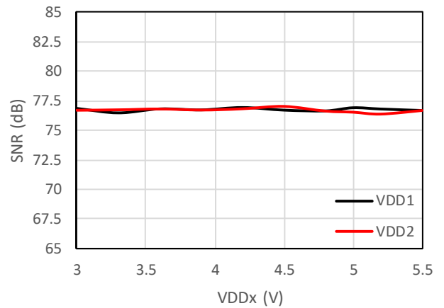
Figure 7-10 SNR vs Supply Voltage @ f_{IN} = 1 \text{ kHz}
