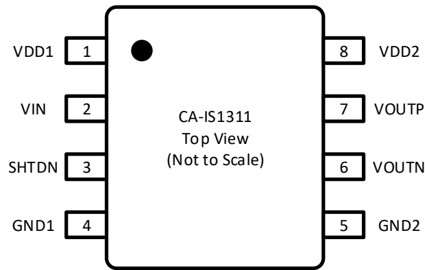
Figure 6-1 CA-IS1311 Top View
