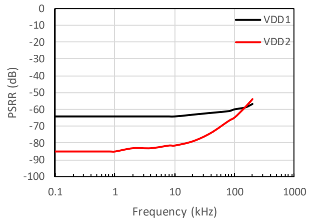
Figure 7-8 PSRR vs Frequency
