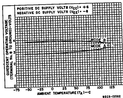
Fig. 6 - Quiescent operating voltage vs temperature.
