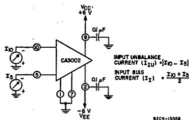
Fig. 5 - Input unbalance current & bias current test circuit.
