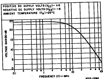
Fig. 8b - Differential voltage gain vs frequency.
