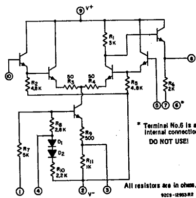
Fig. 1 - Schematic diagram.
