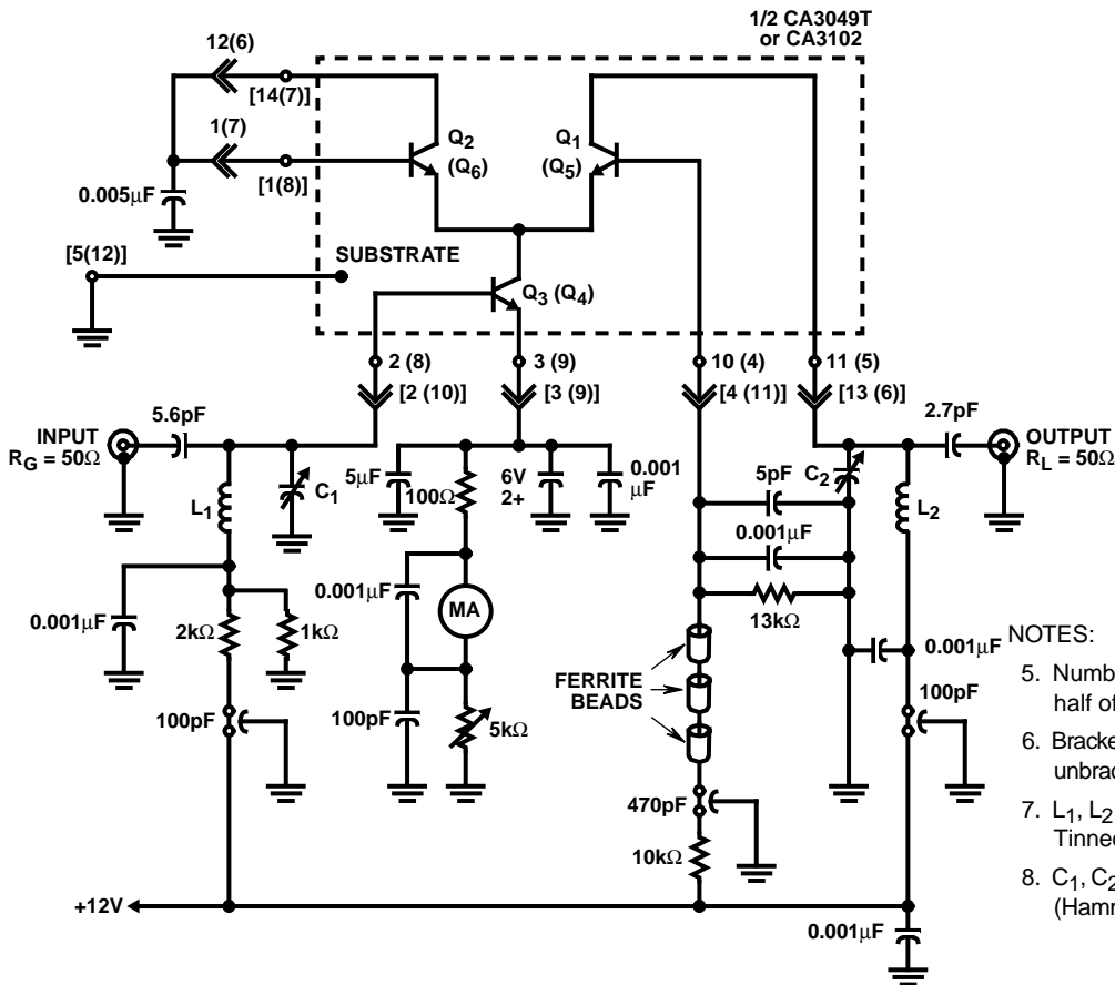
FIGURE 3. 200MHz CASCODE POWER GAIN AND NOISE FIGURE TEST CIRCUIT
