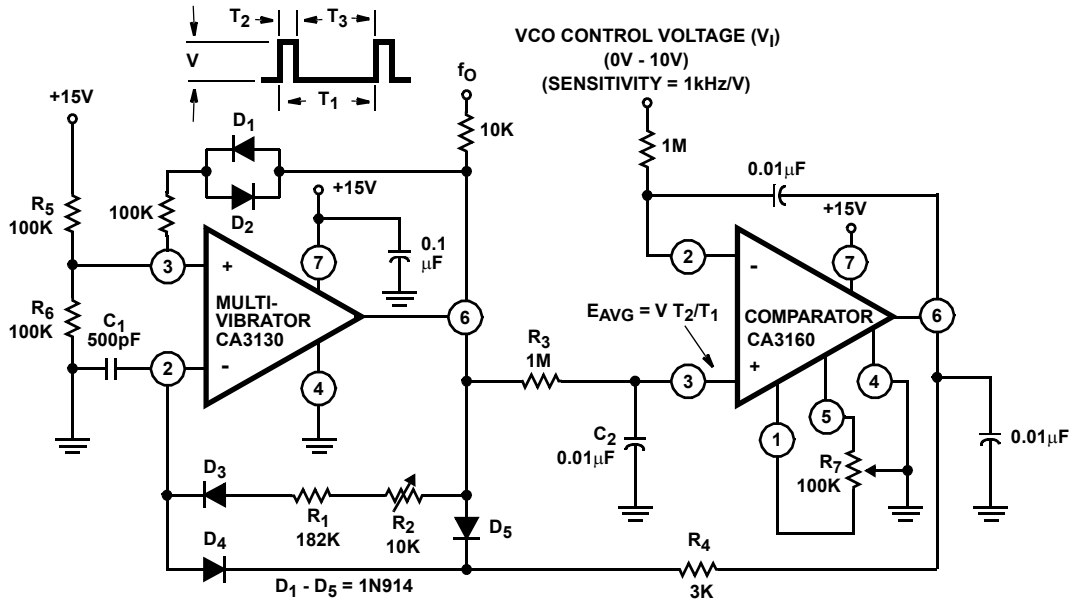
FIGURE 7. VOLTAGE CONTROLLED OSCILLATOR
