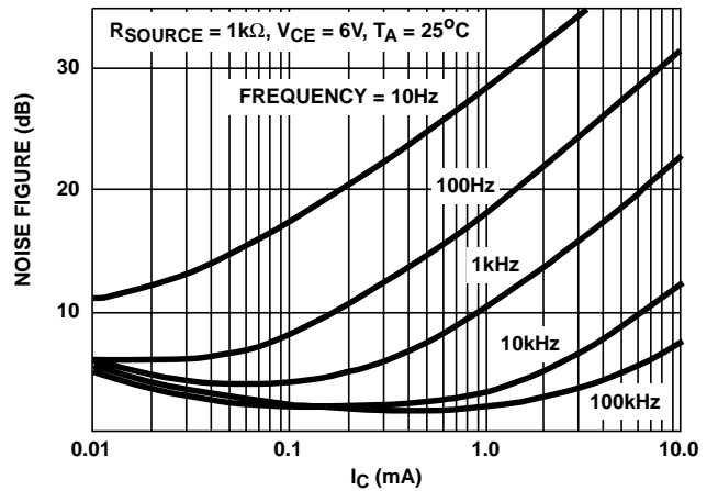
FIGURE 4. NOISE FIGURE vs COLLECTOR CURRENT
