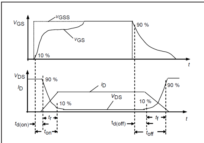
Figure 27. Resistive Switching Time Description
