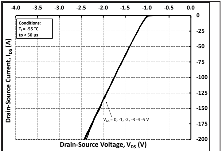
Figure 10. Typical Diode Characteristics T_J = -55^\circ\text{C}
