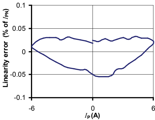
Figure 1: Linearity error
