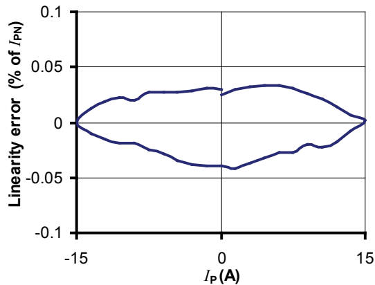
Figure 7: Linearity error
