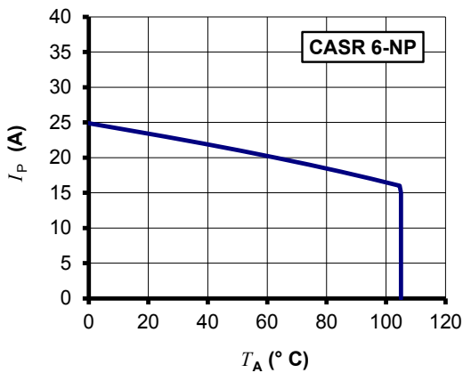
Figure 25: I_P vs T_A for CASR 6-NP
