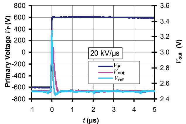
Figure 16: Step response
