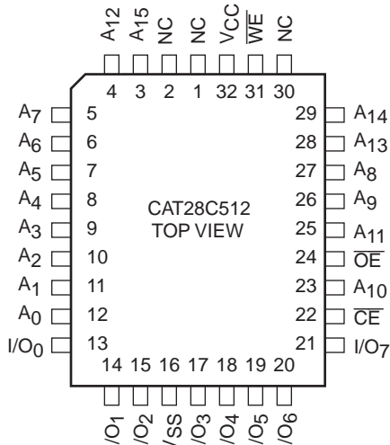
PLCC Package (N)
