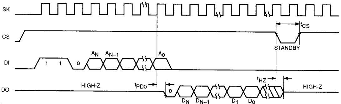
Figure 2. Read Instruction Timing (8) (9)
