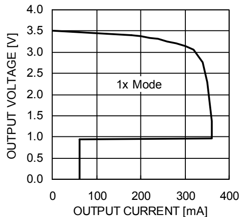
Foldback Current Limit
