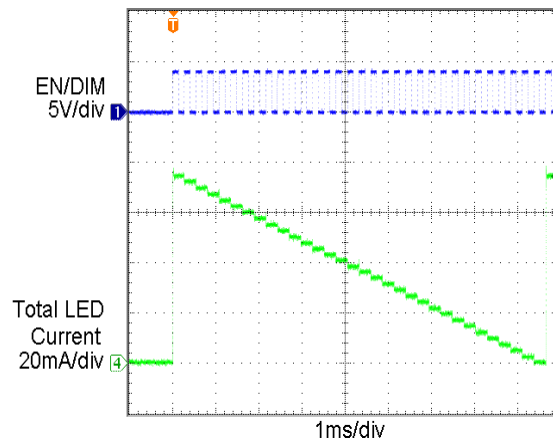
Figure 11. Dimming Levels
