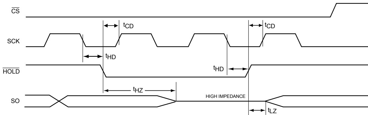
Figure 2. HOLD Timing
