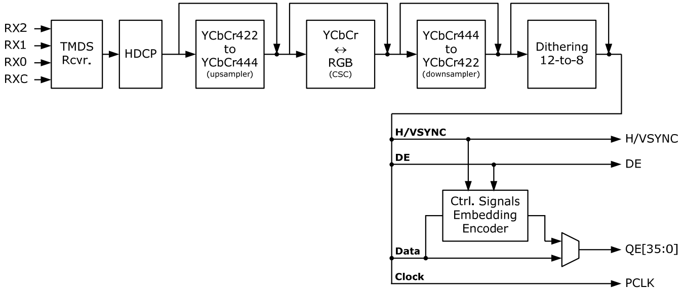
Figure 3. Video data processing flow of the CAT6023A
