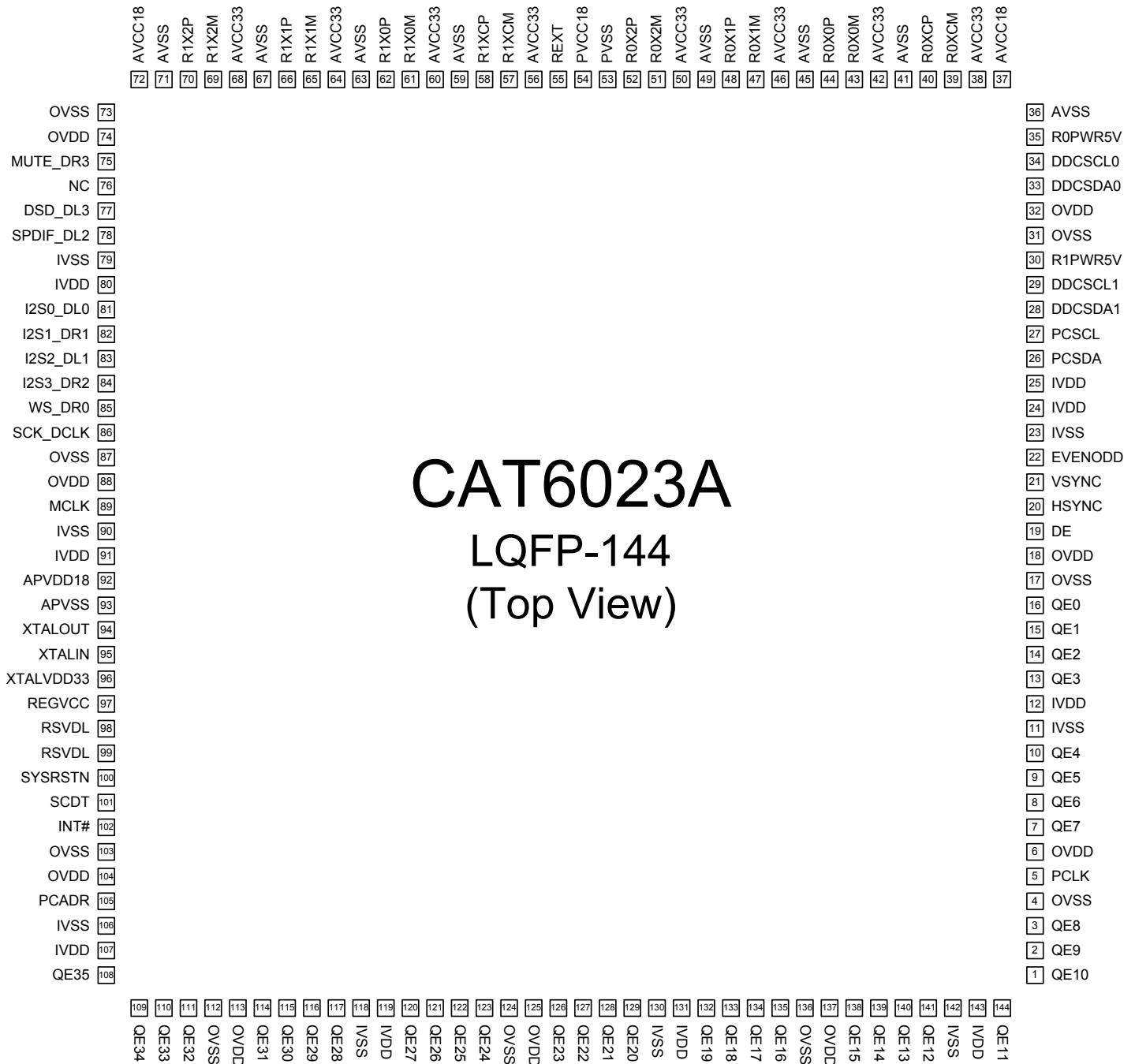
Figure 1. CAT6023A pin diagram
