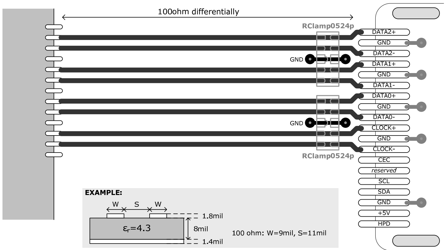
Figure 19. Layout example for high-speed TMD5 differential signals
