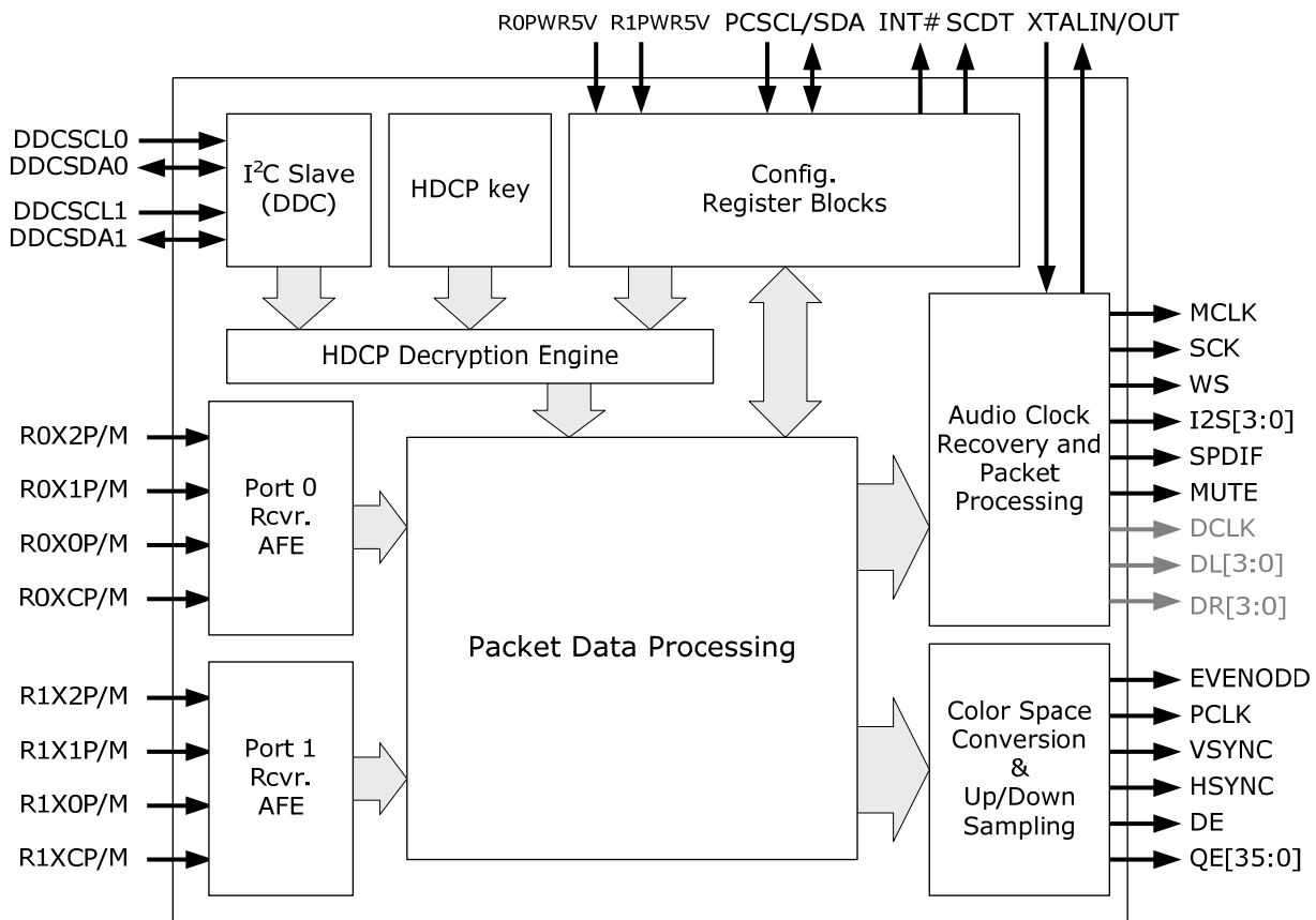
Figure 2. Functional block diagram of the CAT6023A
