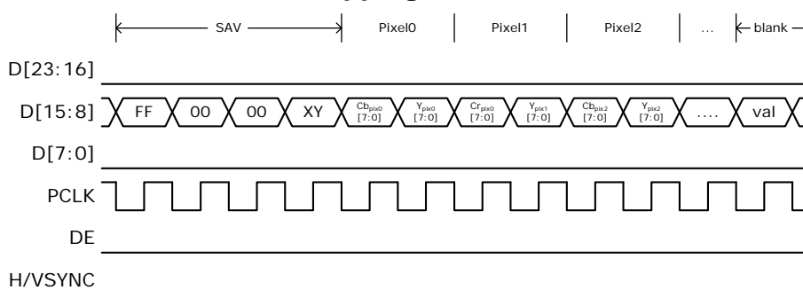
Figure 8. 8-bit CCIR-656
