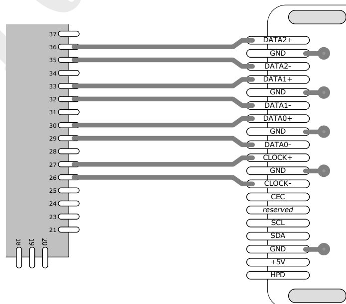
Figure 11. PCB layout example of high-speed transmission lines without ESD diodes
