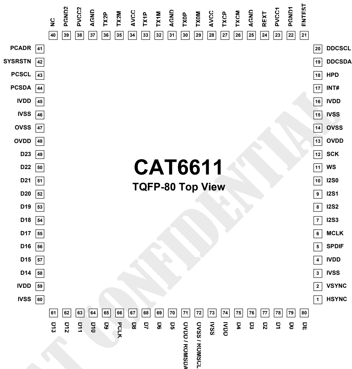
Figure 1. CAT6611 pin diagram
