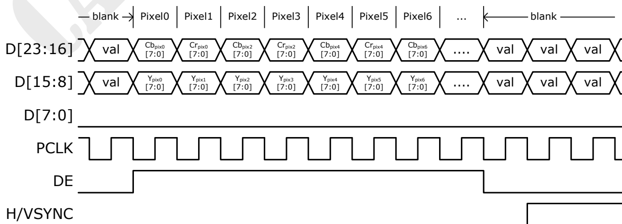
Figure 6. 16-bit YCbCr 4:2:2 with separate syncs
