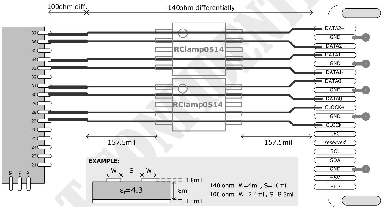
Figure 12. PCB layout guide and example for high-speed transmission lines with RClamp0514
