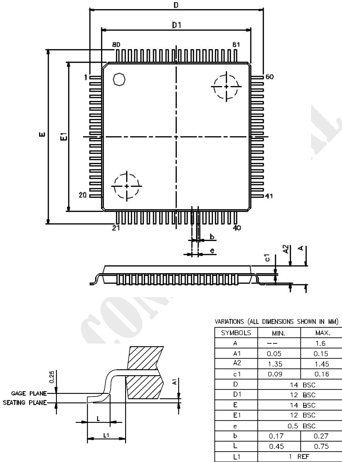
Figure 13. Package dimensions of TQFP-80
