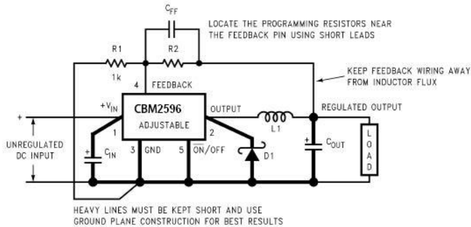
Figure 2. Standard Test Circuit for Adjustable Output Voltage Versions
