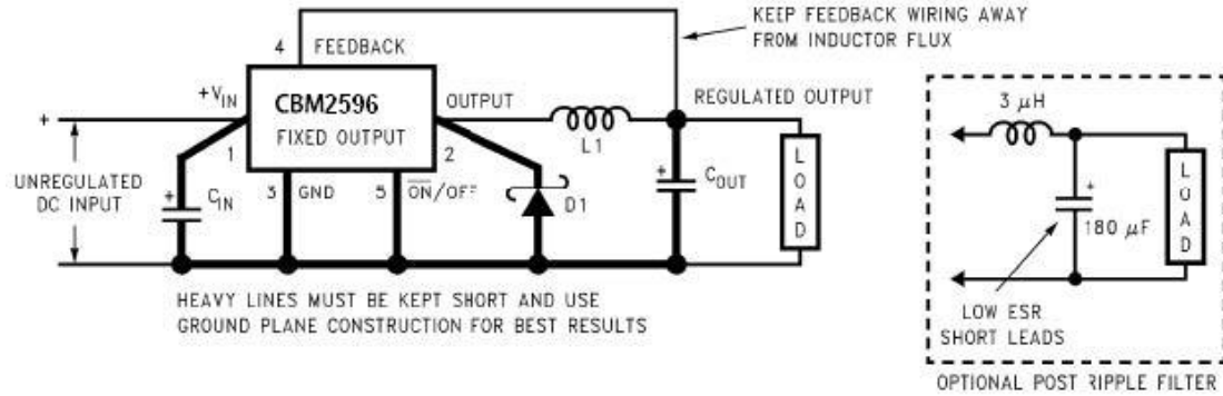
Figure1. Standard Test Circuit for Fixed Output Voltage Versions
