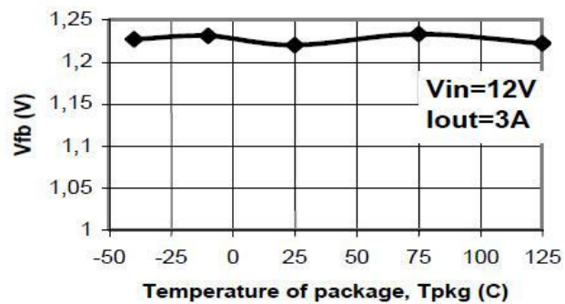
CBM2596-adj Vfb vs Tpkg (TO-220)
