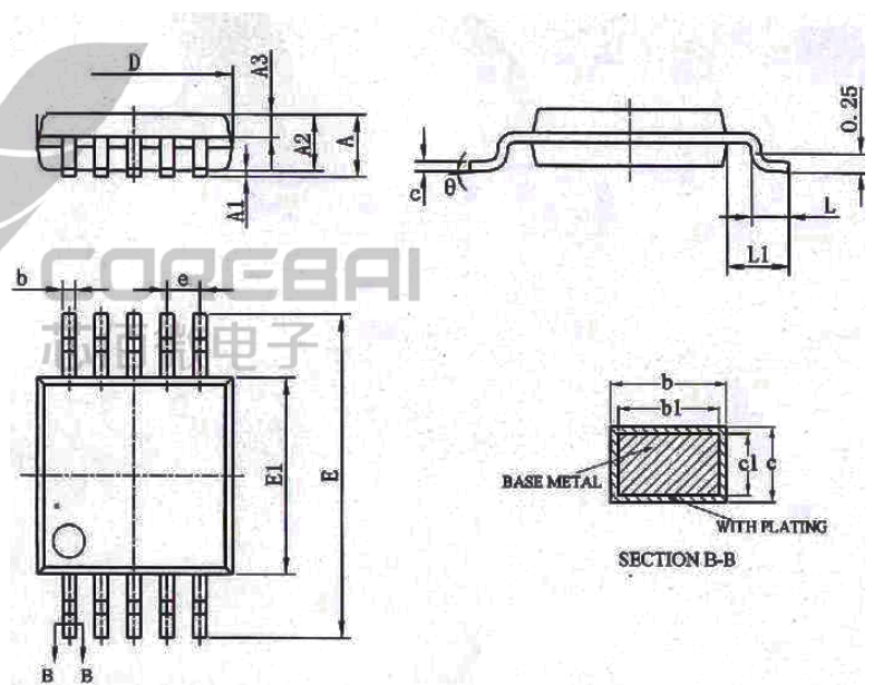
Figure 5 MSOP10L Dimensions shown in millimeters
