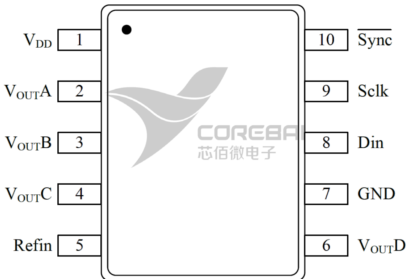
Figure 4. MSOP10L Pin Configuration
