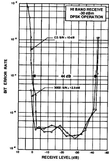
BIT ERROR RATE vs RECEIVE LEVEL
