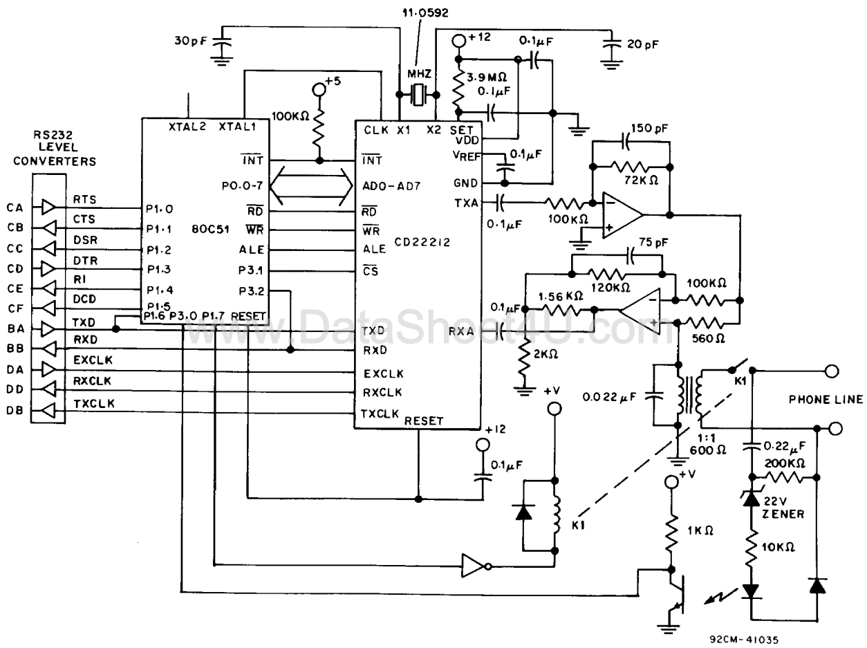
BASIC BOX MODEM
