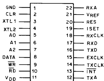
CD22212E1 TERMINAL ASSIGNMENT
