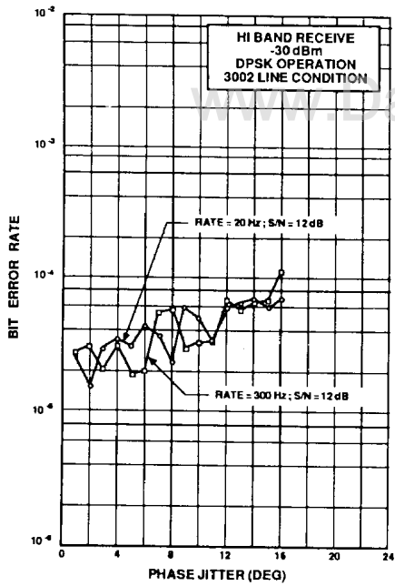
BIT ERROR RATE vs PHASE JITTER
