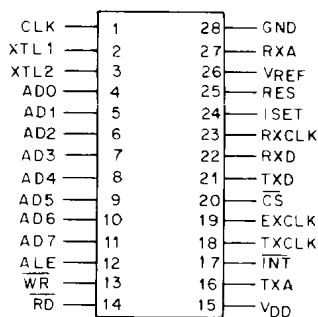
CD22212E TERMINAL ASSIGNMENT
