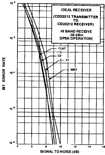
BIT ERROR RATE vs S/N
