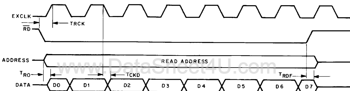
READ TIMING DIAGRAM
