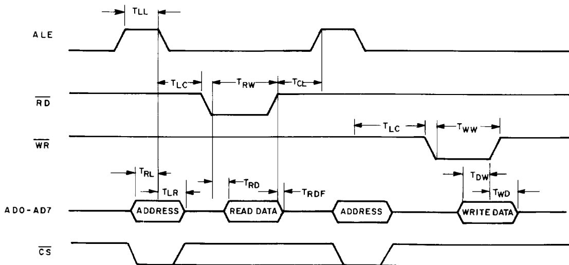
BUS TIMING DIAGRAM
