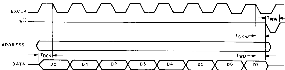
WRITE TIMING DIAGRAM
