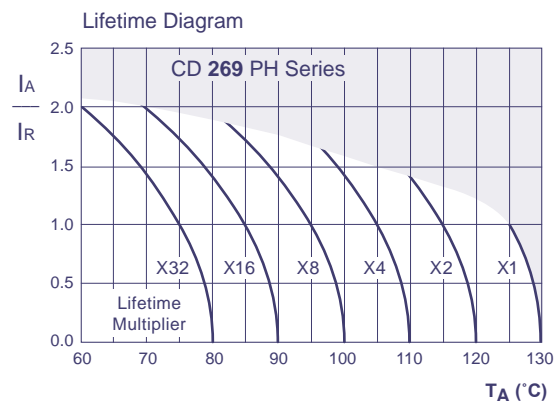
I_A = actual ripple current at 100kHz, I_R = rated ripple current at 100kHz, 125°C Multiplier of Useful Life as a function of ambient temperature and ripple current load
